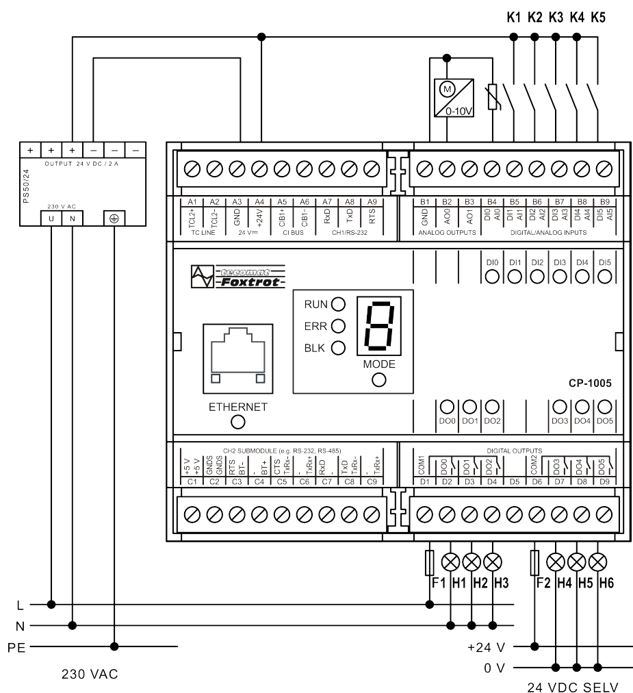
Fig. 4.1 Elementary connection of CP-1005 module
